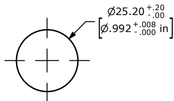
RECOMMENDED PANEL CUTOUT MAX. PANEL THICKNESS 10.0 [.39 in]
